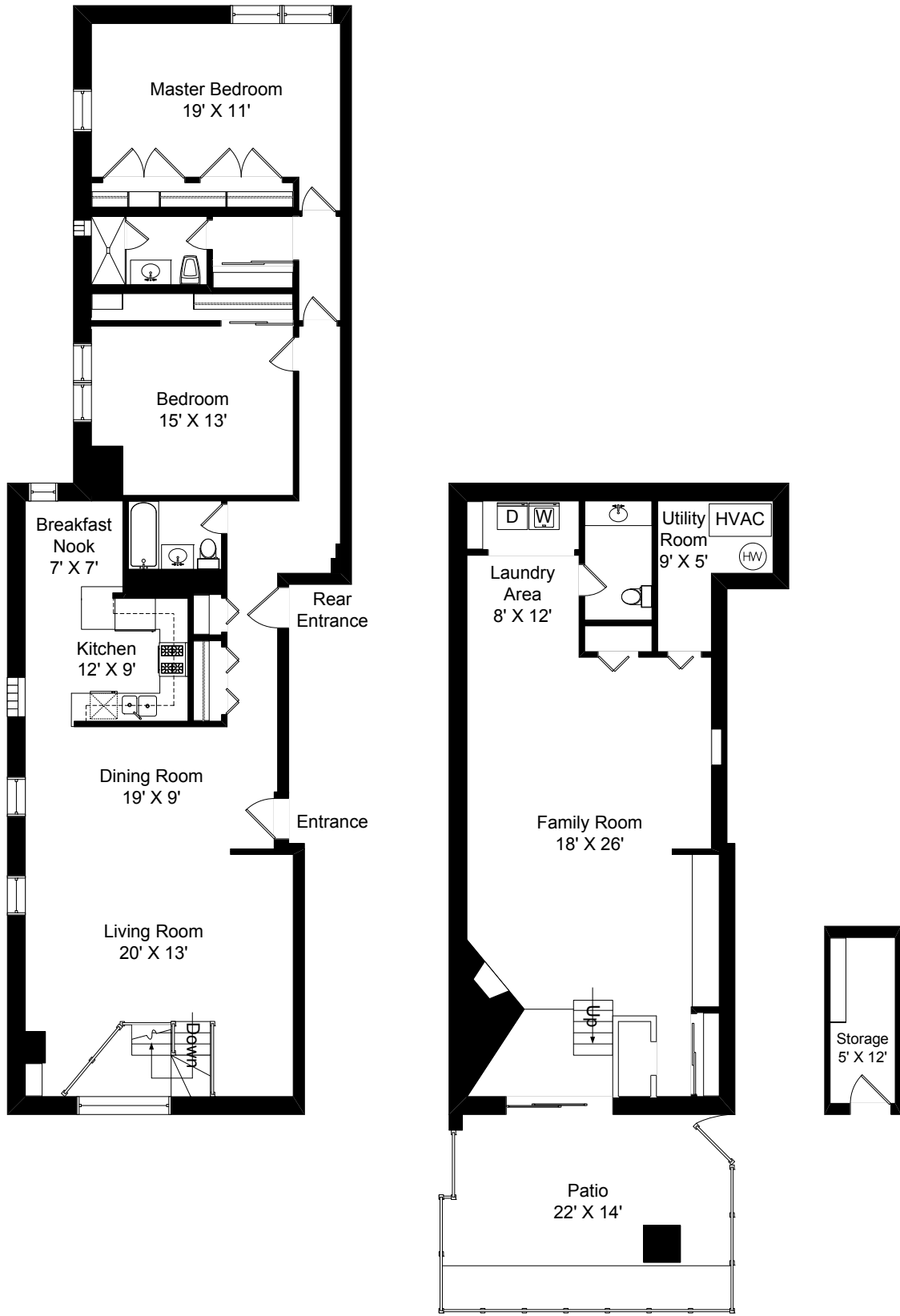
MAIN LEVEL
